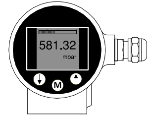
Front view: Transparent cover, option: I (extra price)
