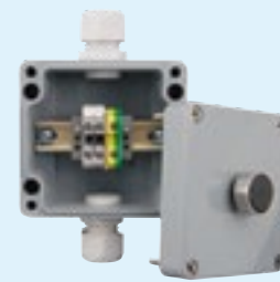
Junction Box FMD (IP67) Art. no. 20069
