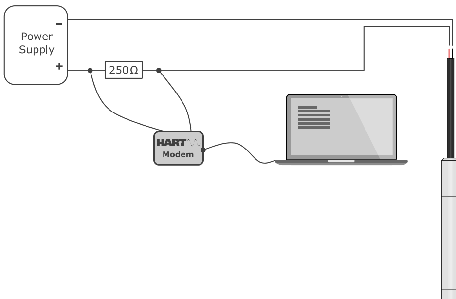
Option 1: HART® Modem connected across the loop resistor.
